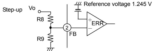
Fig. 25 Feedback Resistor Setting
